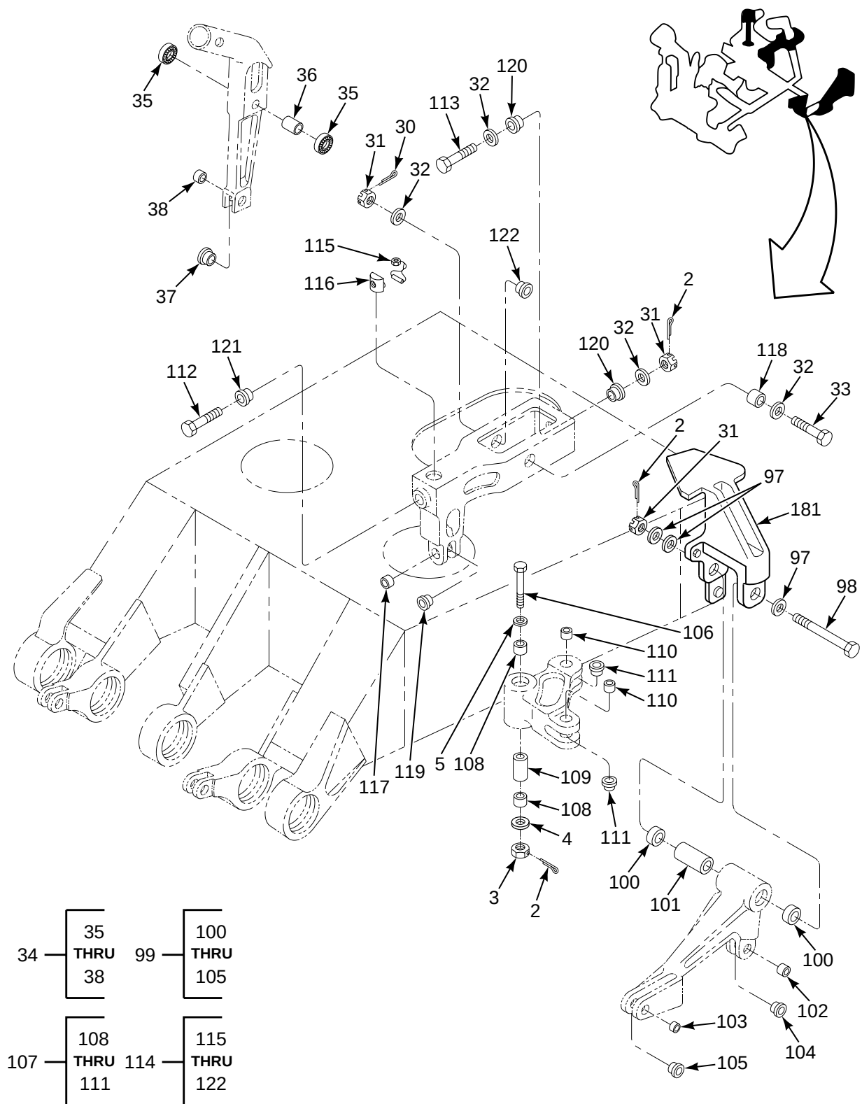
FIGURE 377. CONTROLS ASSY, COPILOT, COCKPIT (SHEET 3 OF 6)
