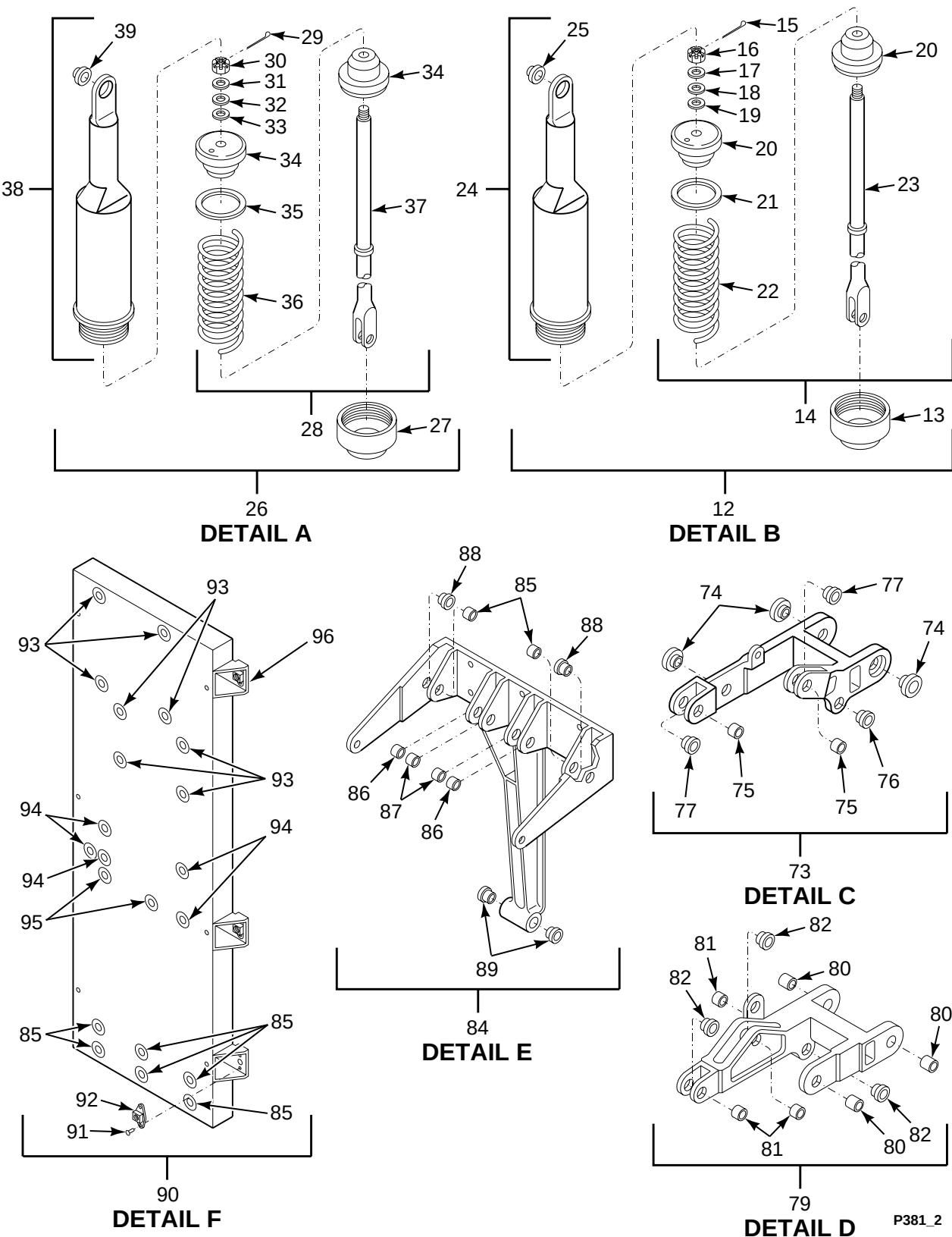
FIGURE 381. CONTROLS, PITCH AND ROLL (SHEET 2 OF 2)
