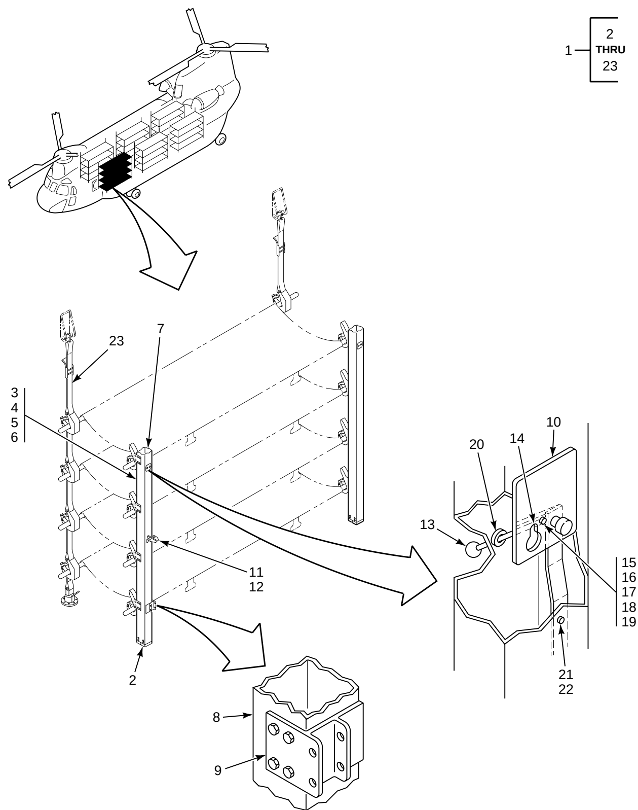
FIGURE 428. LITTER INSTL
