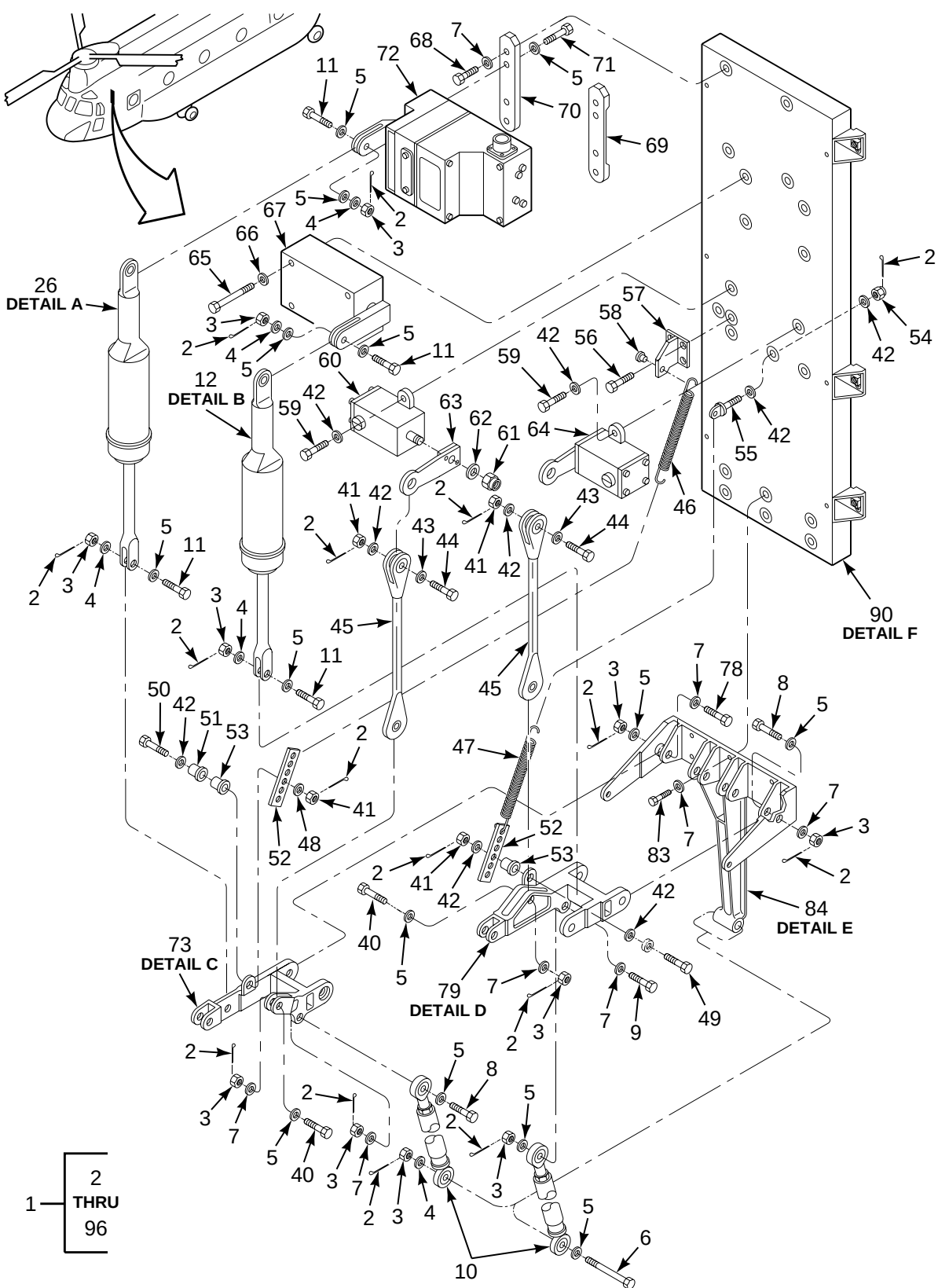
FIGURE 381. CONTROLS, PITCH AND ROLL (SHEET 1 OF 2)
