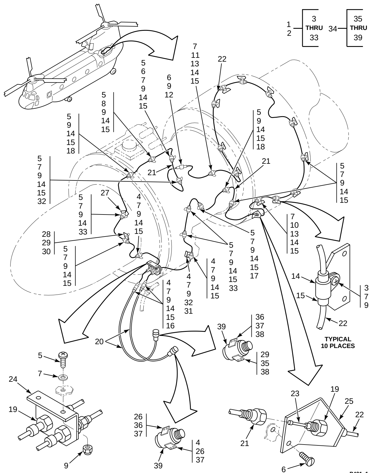
FIGURE 401. FIRE DETECTION SYS, ENGINE COMPARTMENT
