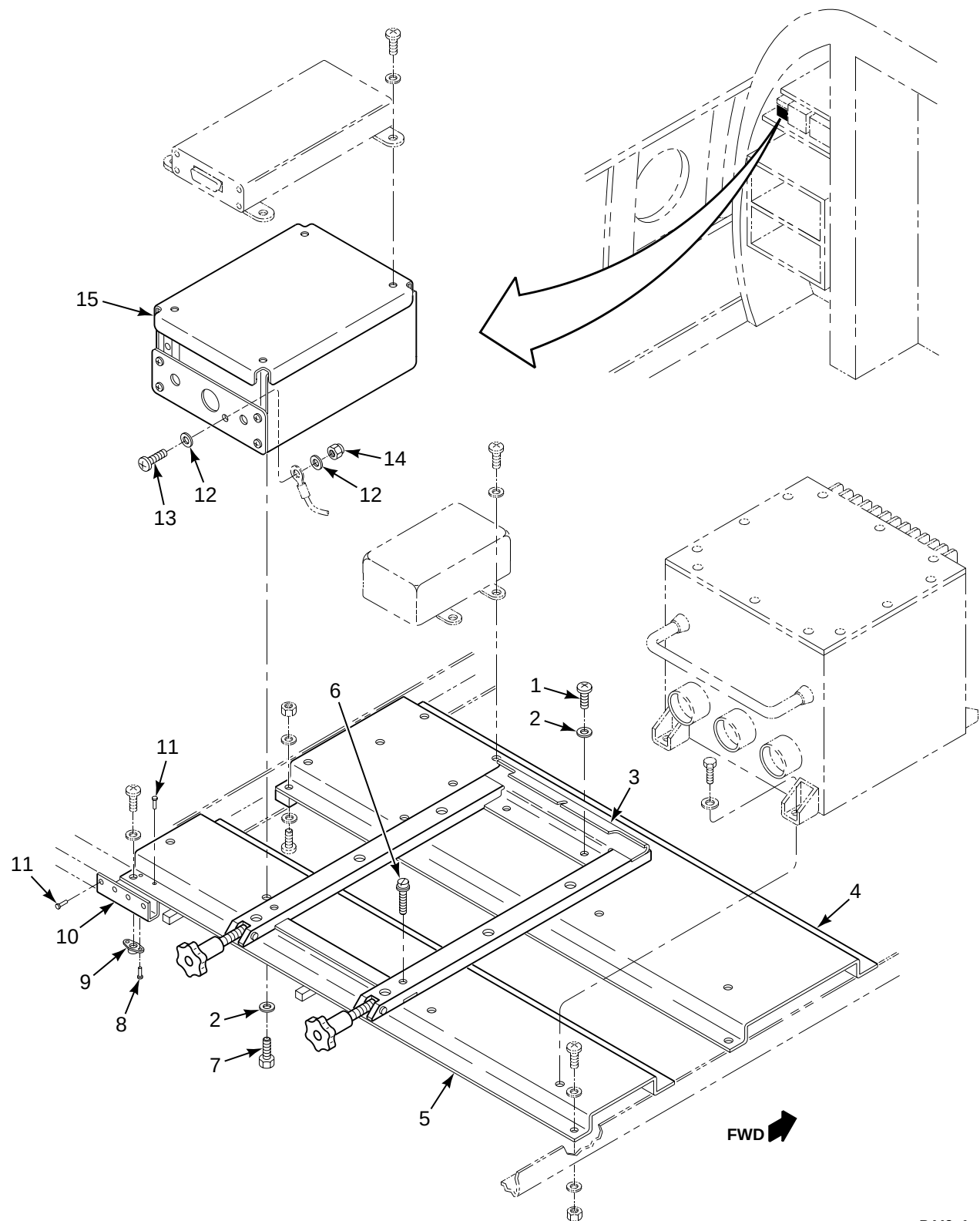
FIGURE 449. GPS RECEIVER AND DATA LOADER INSTL
