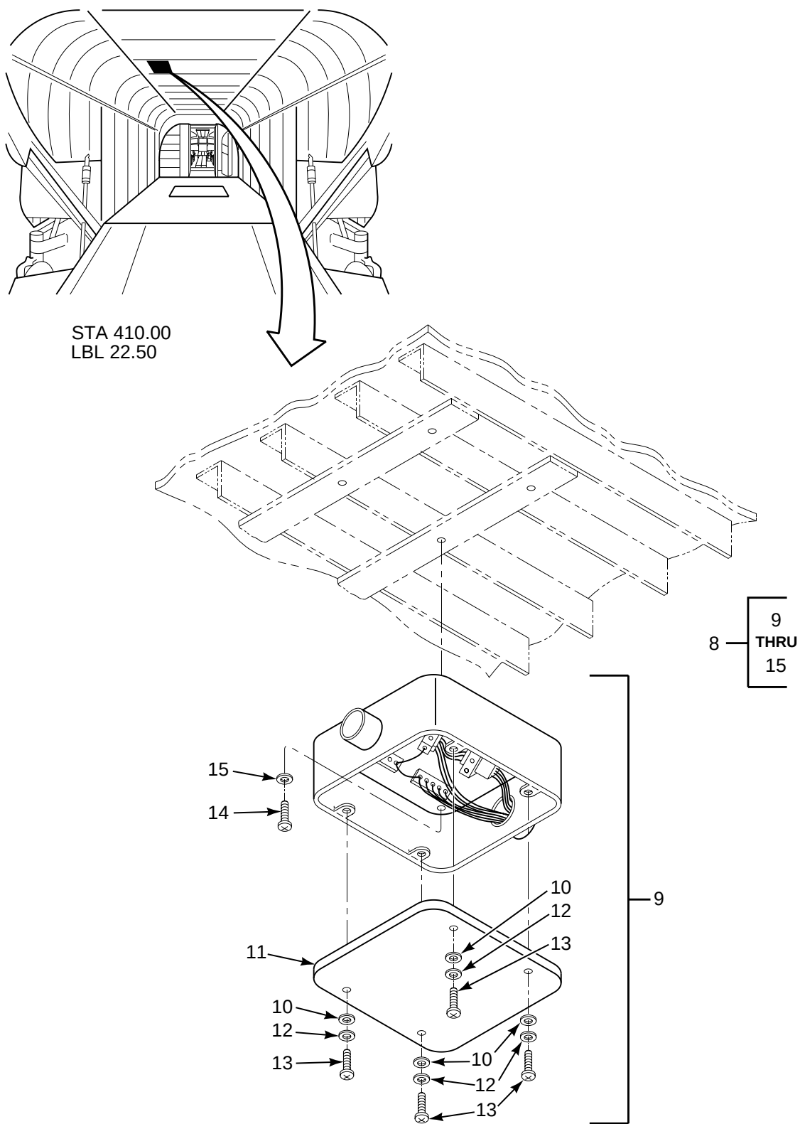
FIGURE 434. AN/ALE-47 COUNTERMEASURES DISPENSER SYSTEM (SHEET 2 OF 8)
