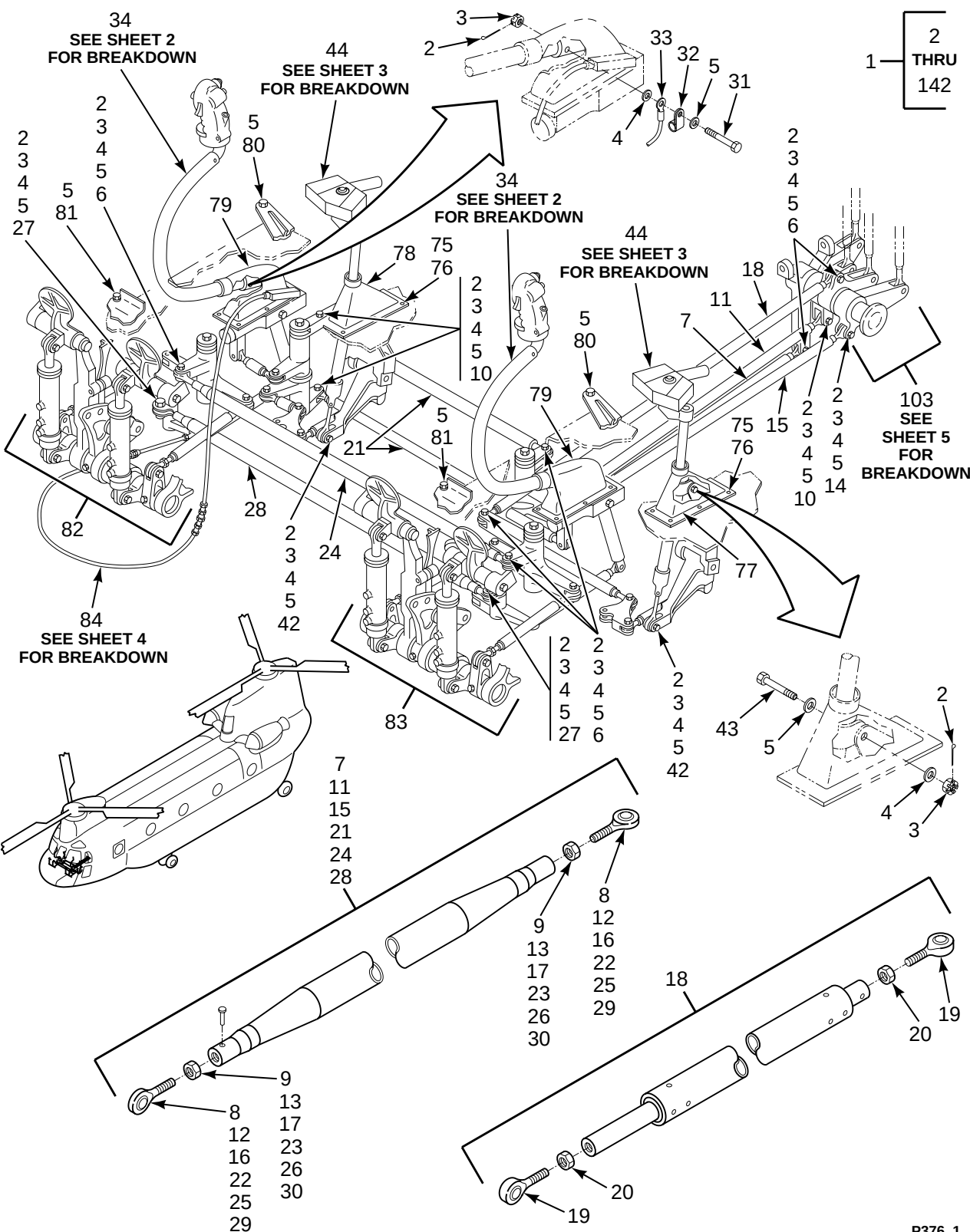
FIGURE 376. CONTROLS INSTL, FLIGHT, COCKPIT (SHEET 1 OF 5)
