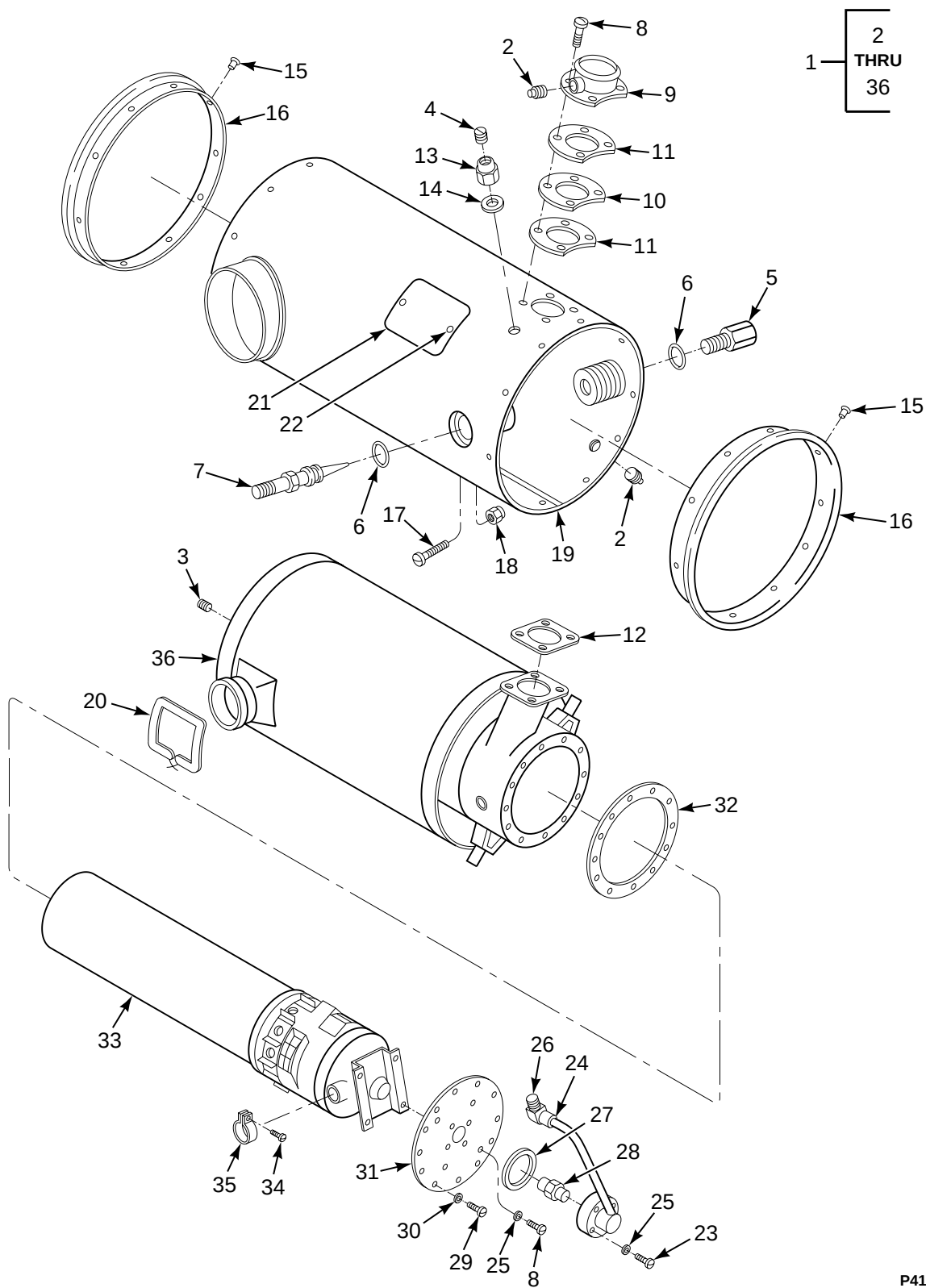
FIGURE 410. HEATER
