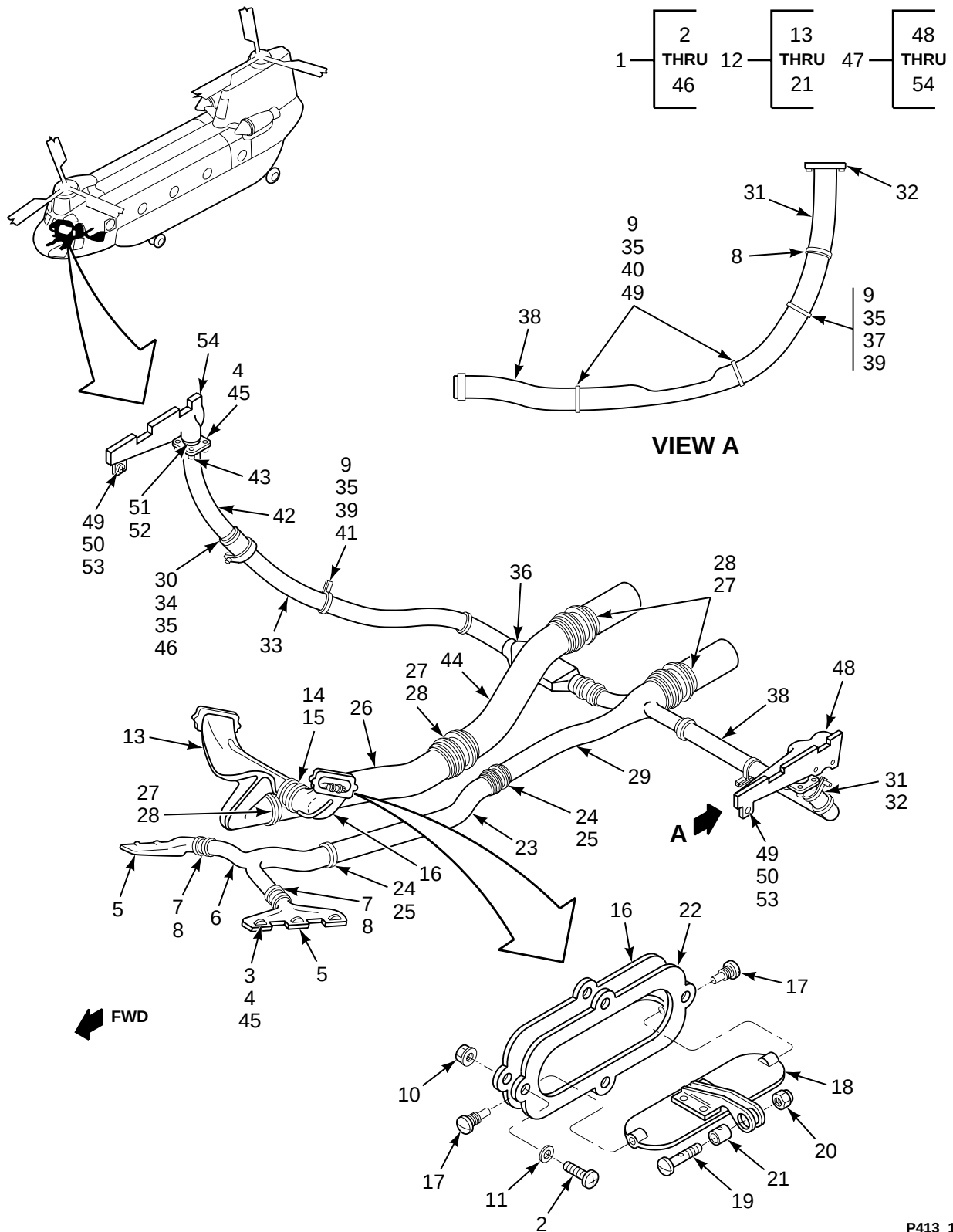
FIGURE 413. DUCT INSTL, COCKPIT
