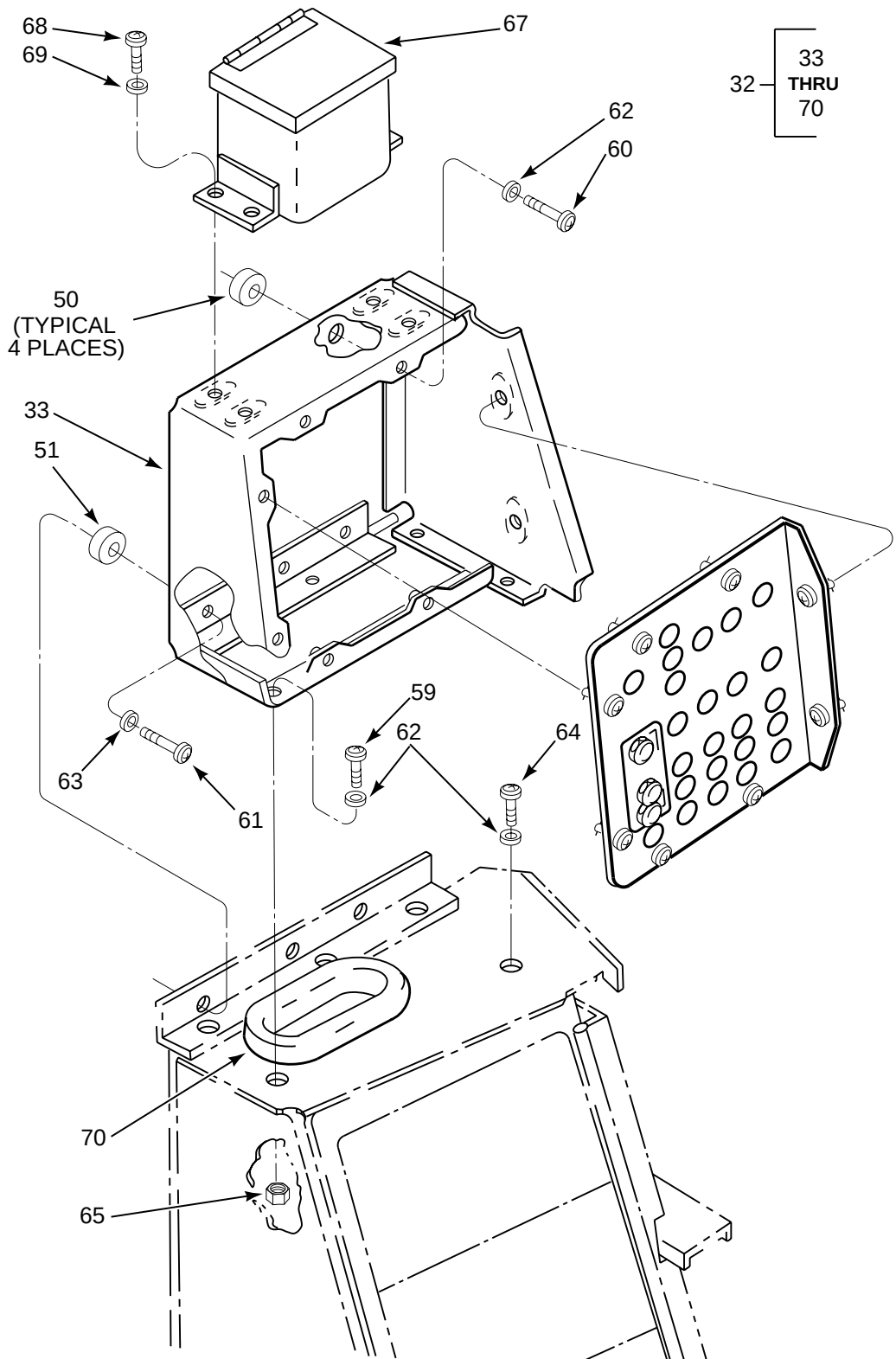
FIGURE 431. ENGINE AIR PARTICLE SEPARATOR (EAPS) INSTL (AIRCRAFT) (SHEET 6 OF 9)
