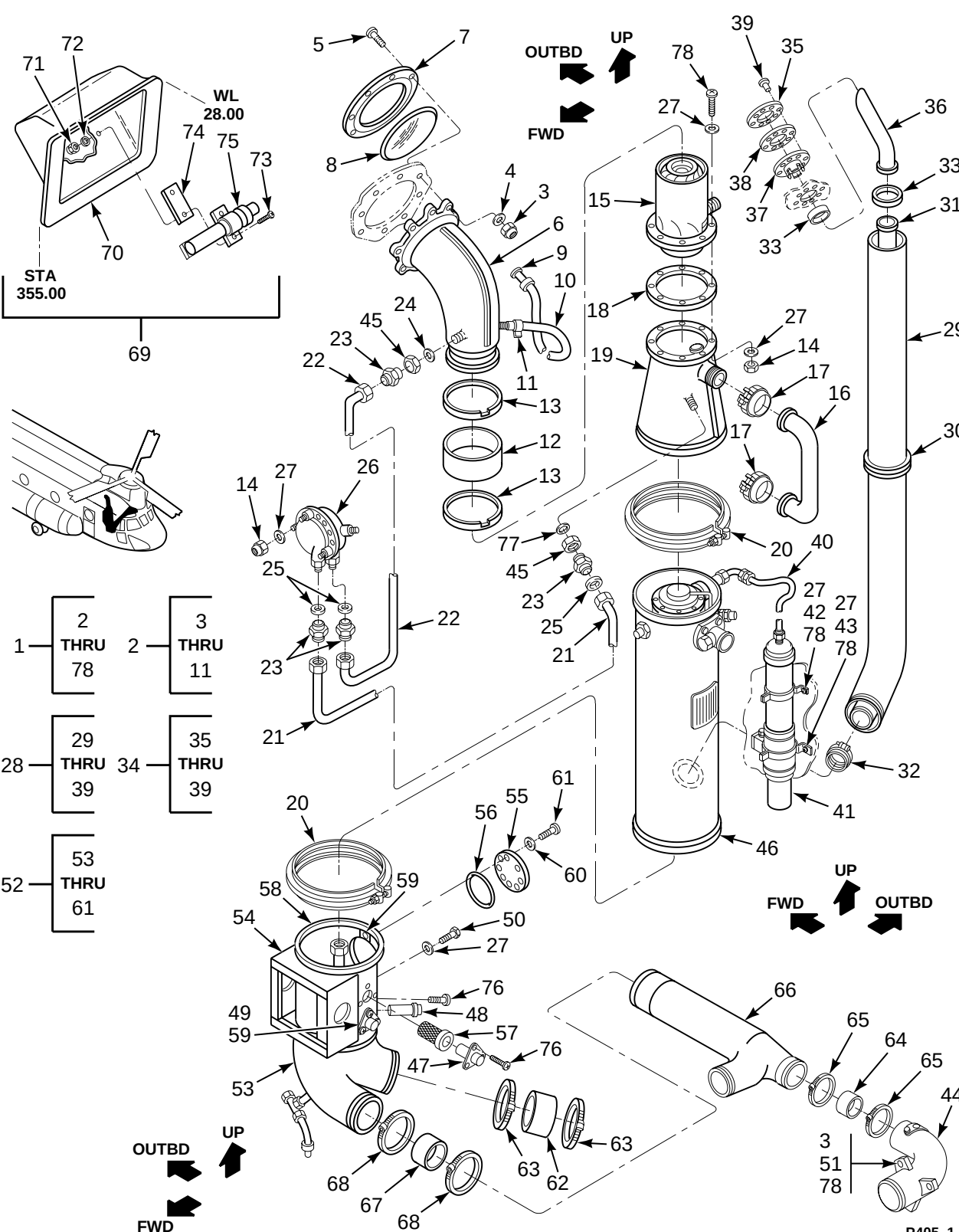
FIGURE 405. HEATER INSTL
