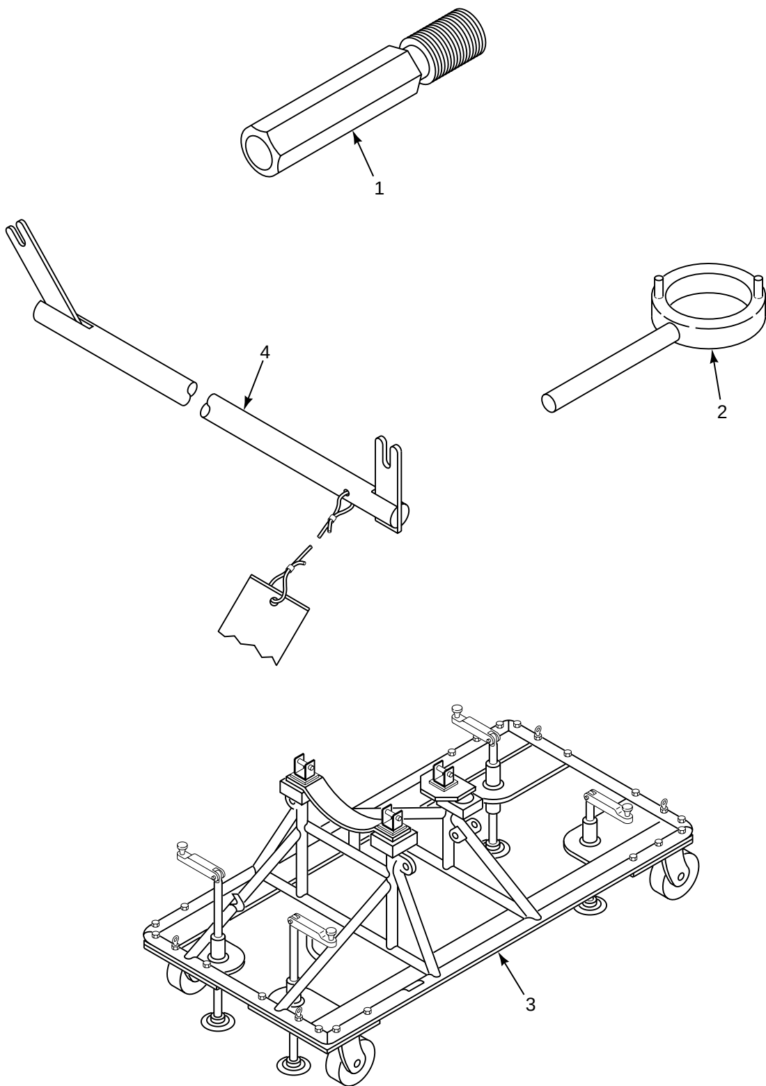
FIGURE A3. AIRFRAME TOOLS
