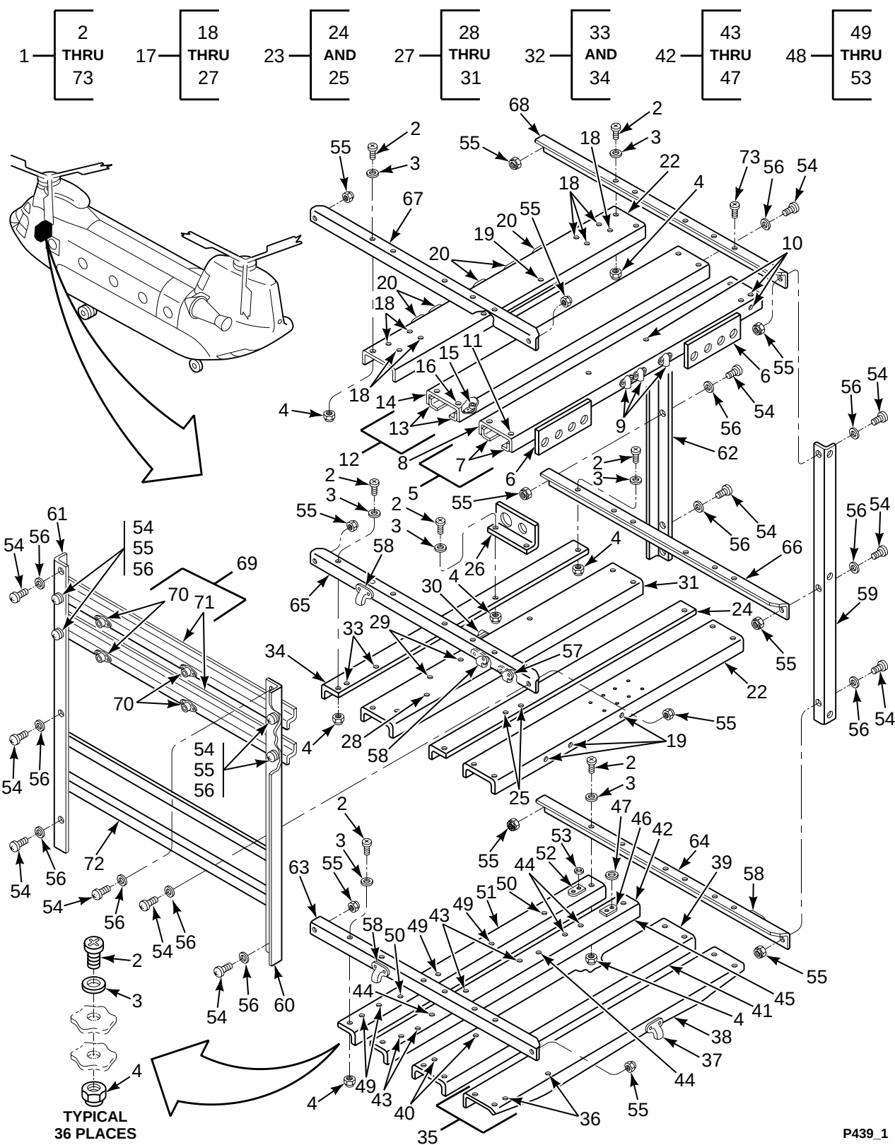
FIGURE 439. RACK DETAIL, ELECTRONIC COMPARTMENT
